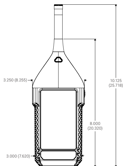
Outline Drawing - Front
